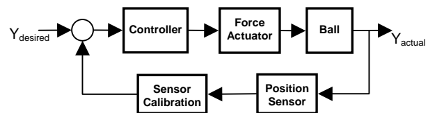
Figure 5: Magnetic Levitation System Block Diagram
