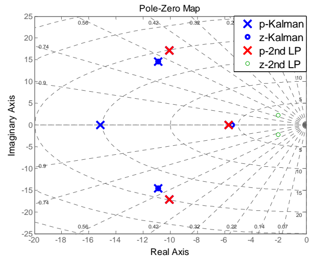
Figure 2. Pole Zero Map for the Feedback Control System
