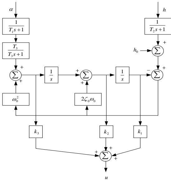
Figure 1. The conventional controller for EMS
