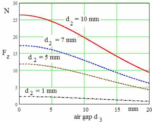
Figure 13. Electrodynamic suspension force as a function of the air gap d_3 for four different thicknesses d_2 = 10; 7; 5; and 1 mm of the secondary bottom at 300 V and 50 Hz. Calculation results on the basis of Lorentz equation [7,8].
