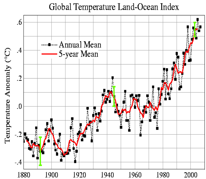
Figure 2. The global temperature land-ocean index for the period 1880 to 2007. The dotted black line is the annual averages and the smoother red line is the five-year running averages. The green bars are estimated errors. NASA GISS (2008).
