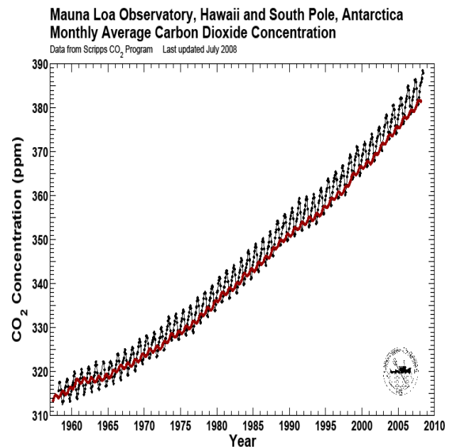
Figure 1. CO 2 concentrations measured at Mauna Loa (upper black curve) and at Antarctica (lower red curve). Scripps (2008).
