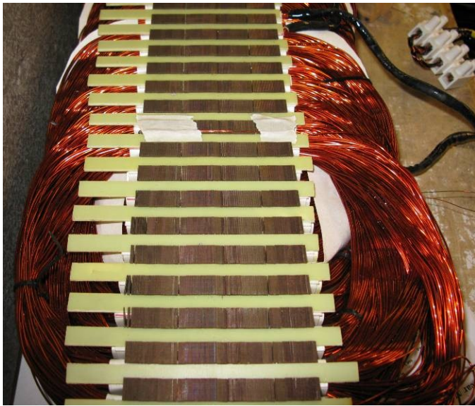
Figure 3. Double sided stator launch assembly
