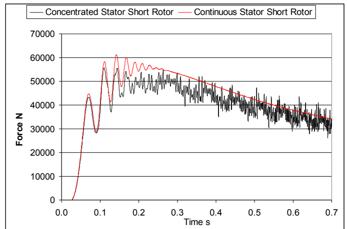
Figure 10. Force-time curve for offset launcher
