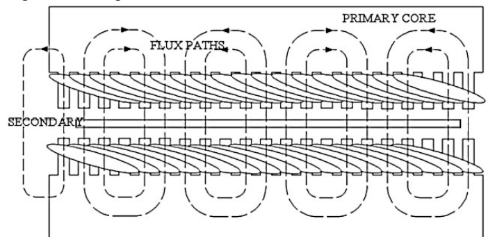
Figure 2. Flux paths in a double sided linear induction motor
