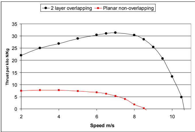
Figure 5. Comparison of stator performance using a plate rotor
