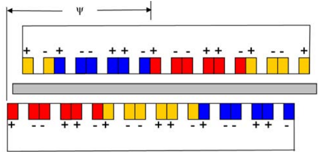
Figure 7. Machine using 9 coil 8/10 pole stators
