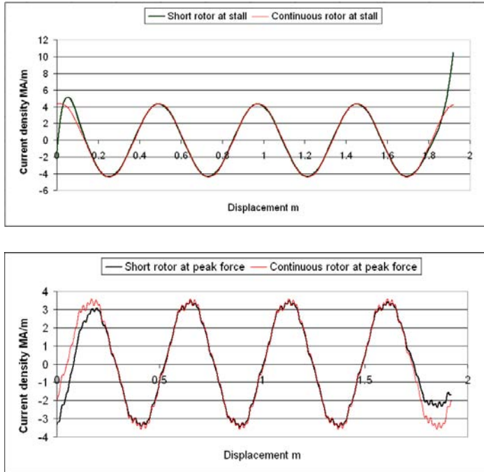
Figure 8. Short rotor plate currents
