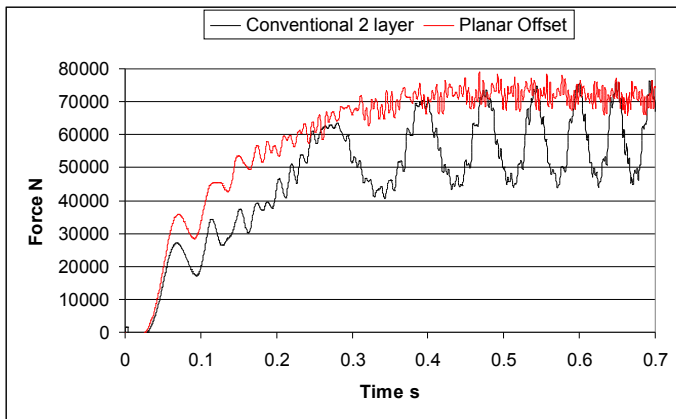
Figure 12. Launcher comparison force-time
