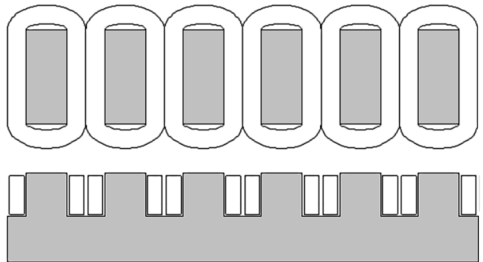
Figure 4. Planar winding construction
