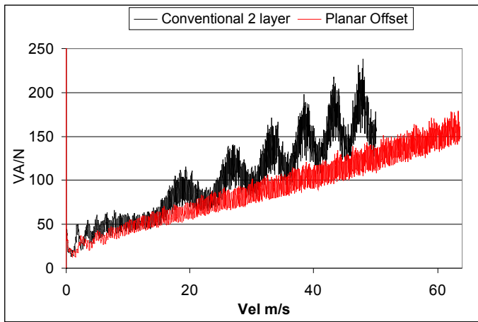
Figure 13. Launcher comparison VA/N-time
