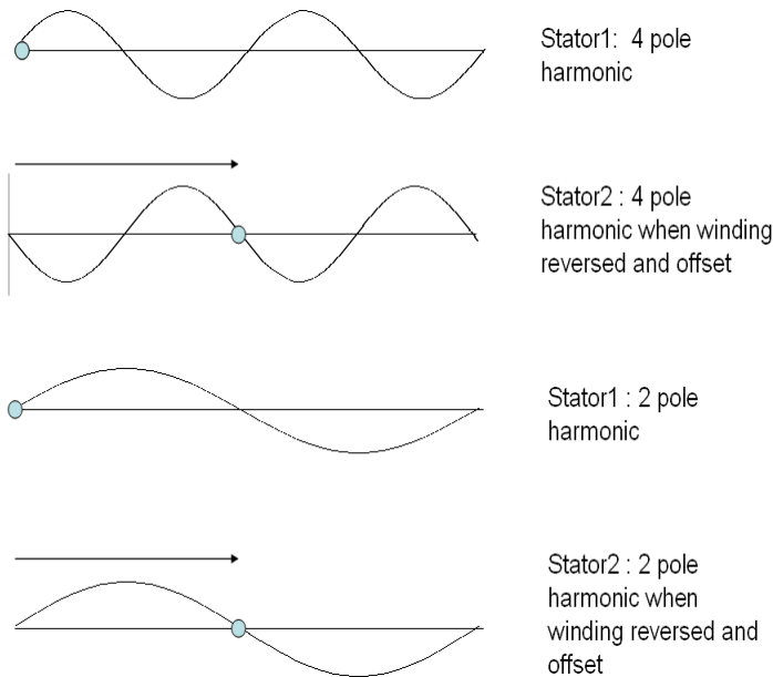
Figure 6. Harmonic cancellation of the 4 pole field and reinforcement of the 2 pole field
