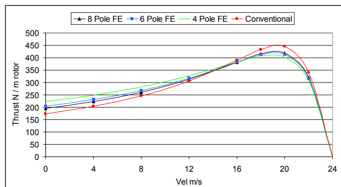
Figure 9. Short rotor thrust speed curves
