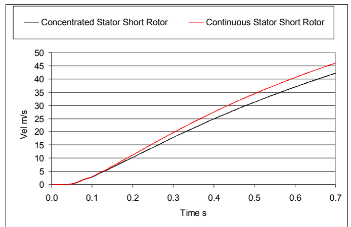
Figure 11. Speed-time curve for offset launcher
