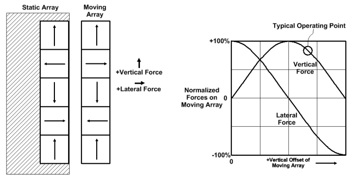
Figure 3: Shear-force levitator
