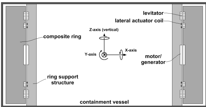
Figure 5. Power Ring cross section
