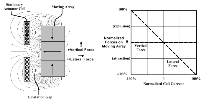
Figure 4: Stabilization actuator
