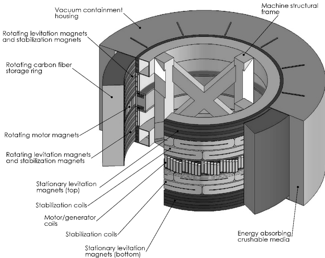
Figure 7: Utility Power Ring
