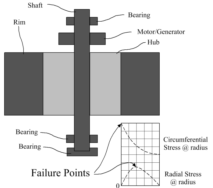
Figure 2: Flywheel structure
